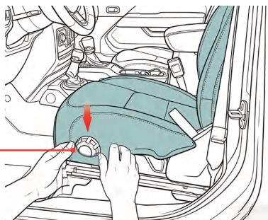
Fit the opening on the side of the driver's seat cover around this knob. If the passenger seat does not have this knob, skip this step.
